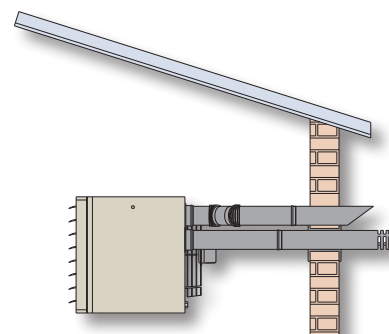
Separate combustion air and flue pipes (type C12) for applications where wall thickness exceeds maximum length shown in flue dimension table
